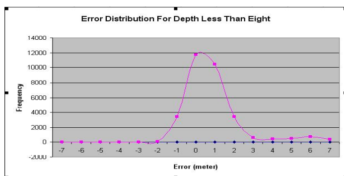
Error distribution graph for differences in measured depth and derived bathymetry depth for depths less than eight metres.
